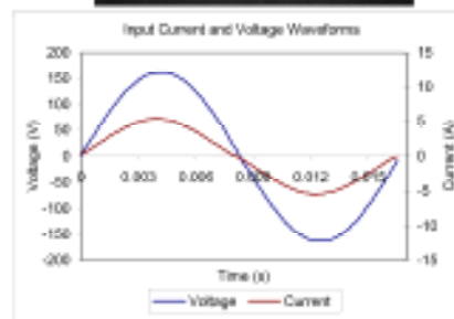
Input AC Current Waveform (THD = 8.85%, 50% Load)
